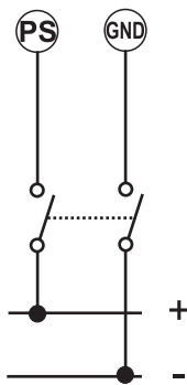
Fig. 12 Power supply
