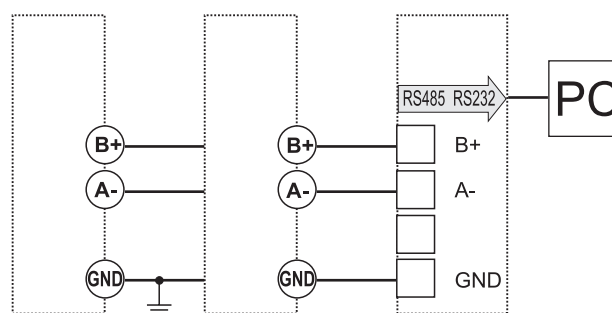
Fig. 4 RS485
